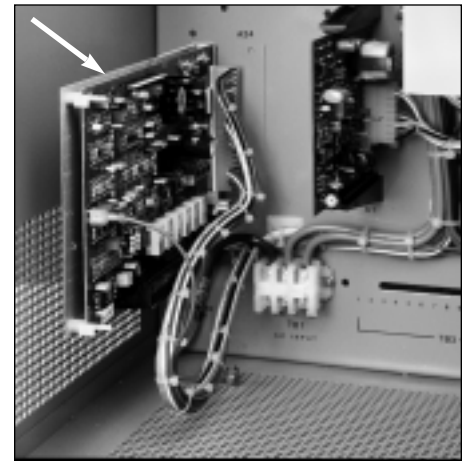
Typical internal construction detail showing Combined Alarm – Status Charger Monitor option
