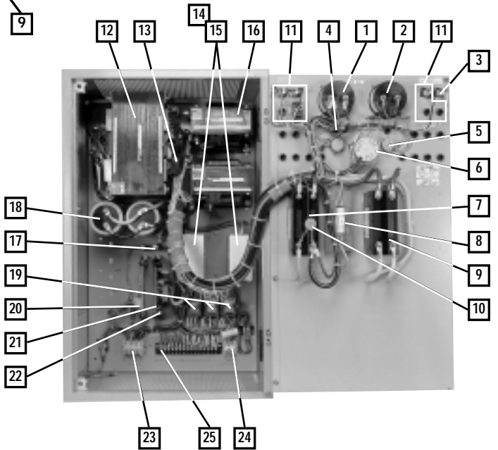
STYLE 1B CABINET CONSTRUCTION
