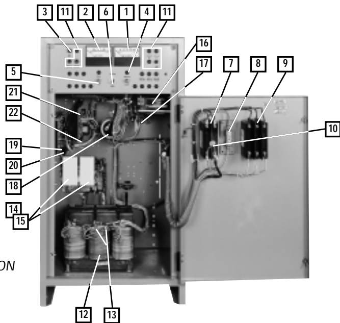
STYLE 1B CABINET CONSTRUCTION
